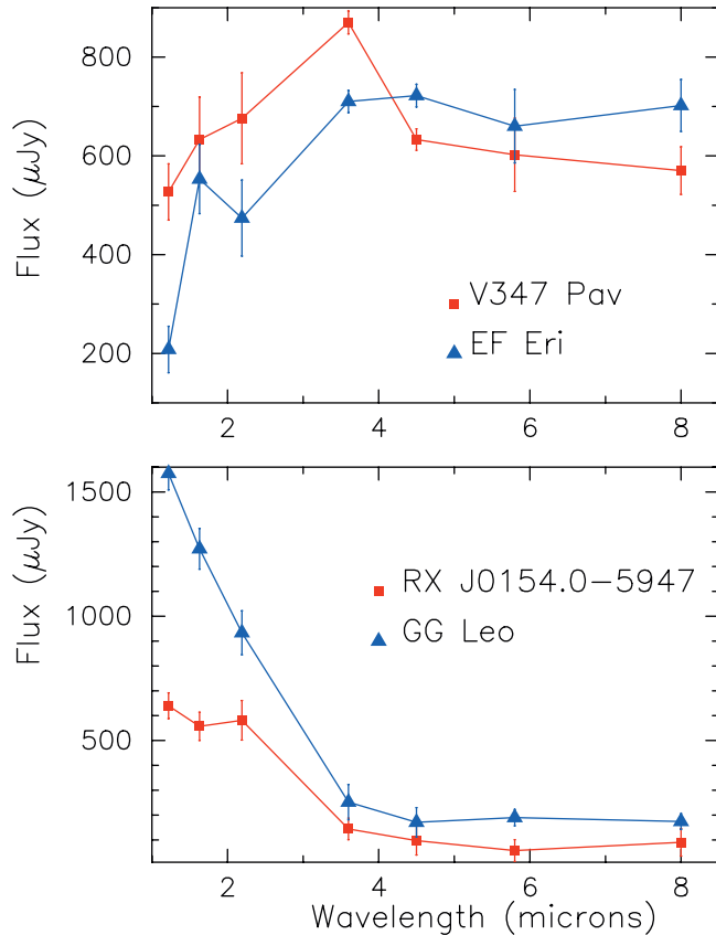
FIG. 1.— Spitzer IRAC photometric observations at 3.6, 4.5, 5.8, and 8.0 \mu\text{m} and 2MASS JHK , photometry for the Polars EF Eri and V347 Pav (top) and GG Leo and RX J0154.0–5947 (bottom).
